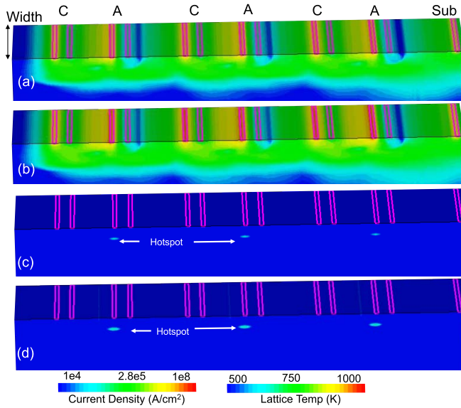
Fig. 5. (a) and (b) Conduction current density ( A/cm^2 ) and (c) and (d) lattice temperature (K) extracted at the end of very fast ( RT = 5 ns) stimulus for (a) and (c) lower stress level ( Q = 0.8 \times 8.52e-9 C) and (b) and (d) higher stress levels ( Q = 1.4 \times 8.52e-9 C). Uniform turn-on of all the fingers is observed for very fast stimulus.
