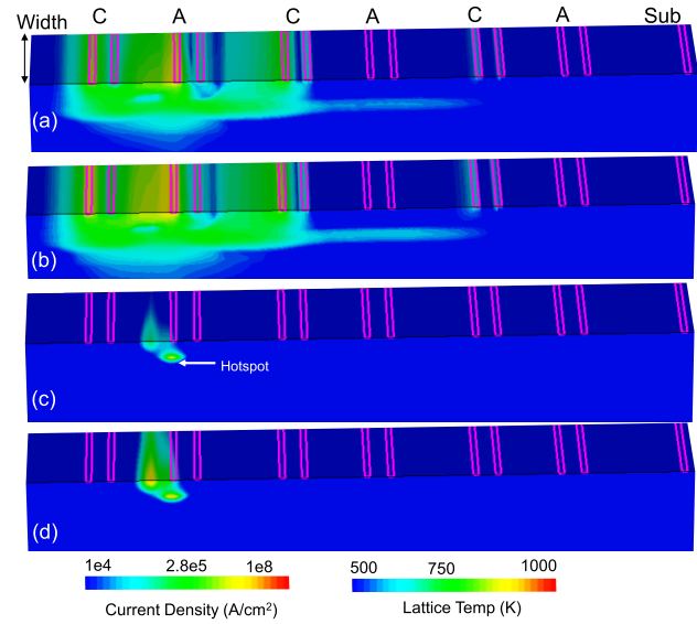
Fig. 7. (a) and (b) Conduction current density ( A/cm^2 ) and (c) and (d) lattice temperature (K) extracted at the end of the ultraslow ( RT = 50 ns) stimulus for (a) and (c) lower stress level ( Q = 0.8 \times 8.52e-9 C) and (b) and (d) higher stress levels ( Q = 1.4 \times 8.52e-9 C).
