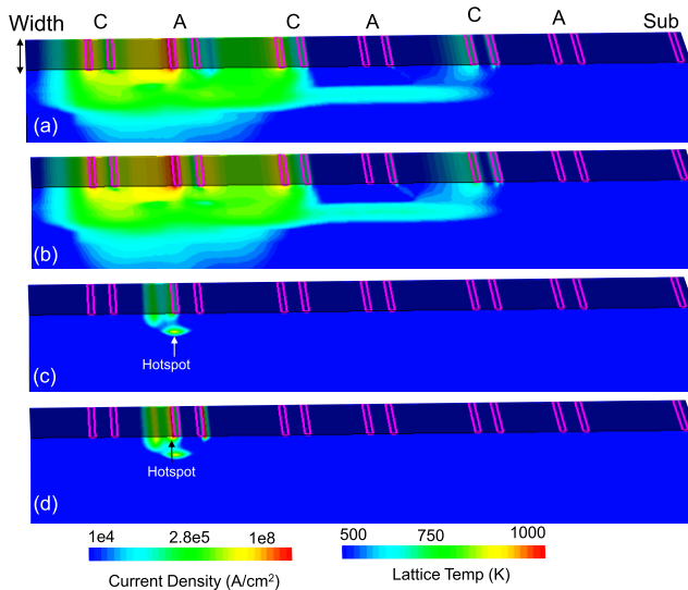
Fig. 6. (a) and (b) Conduction current density ( A/cm^2 ) and (c) and (d) lattice temperature (K) extracted at the end of fast ( RT = 10 ns) stimulus for (a) and (c) lower stress level ( Q1 = 0.8 \times 8.52e-9 C) and (b) and (d) higher stress levels ( Q2 = 1.2 \times 8.52e-9 C). Nonuniform turn-on can be seen across fingers.
