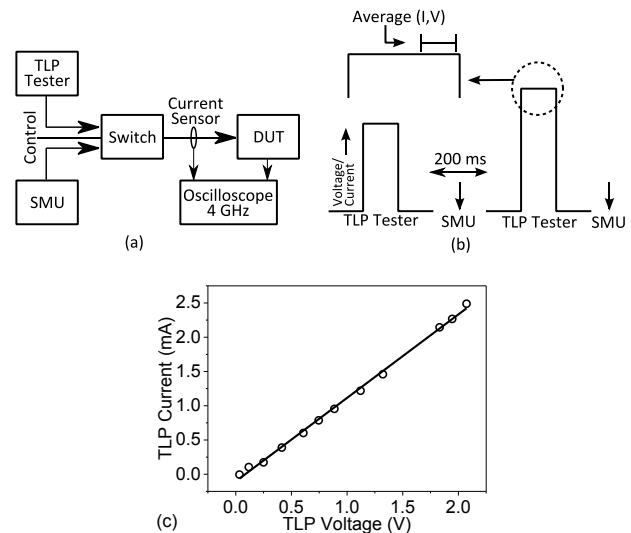
Figure 1: (a) Experimental setup for emulating ESD stress through MWCNTs. All cables and ports are 50 \Omega matched. (b) Analysis technique: Low bias ( 500 \text{ mV} ) DC current is extracted after each pulse, while the response towards pulsed voltage is averaged in a window from 70% to 90% of the pulse width. (c) TLP characteristic of an SMD resistor. The curve shows linear behavior in both sub-mA and mA range.
