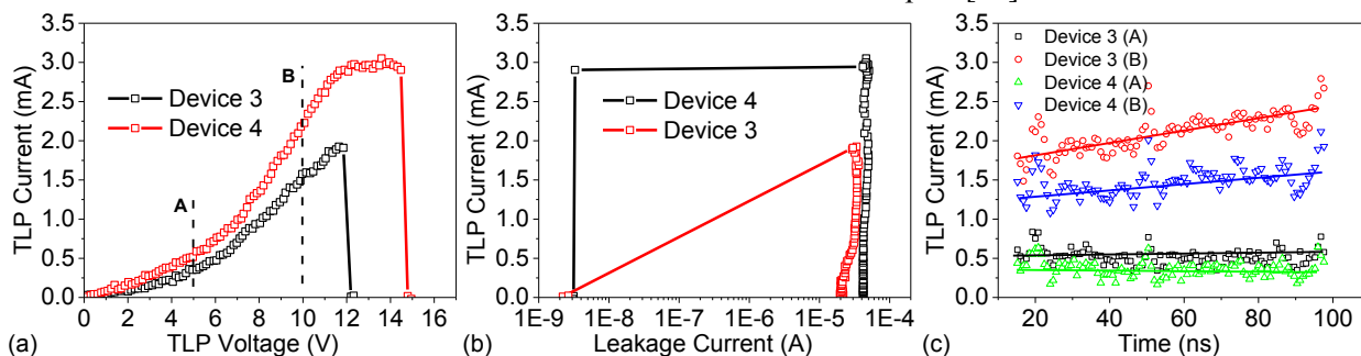
Figure 6: (a) TLP characteristics of substrate-supported tubes (b) change in low-bias DC current w.r.t. TLP current (c) Transient waveforms at two different TLP voltages marked in (a). Unlike suspended tubes, the transient rise in collapsed tubes is relatively less pronounced and happens at much higher voltage.
