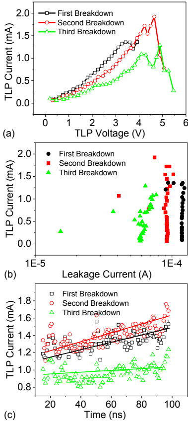
Figure 10: (a) ESD current through inner shells; (b) fall in current through nanotubes after a particular TLP current, indicates breakdown of few outer shells; (c) Change in ESD current with time. Note that current through outer shells (first and second breakdown) increases with time, while current through inner shells (third breakdown) remains constant with time. Transient data is shown for TLP voltage of 4 V.
