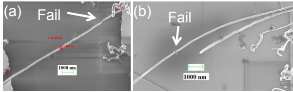
Figure 7: (a) SEM image of Device 3 (b) SEM image of Device 4. Both the devices are resting on \text{SiO}_2 .
