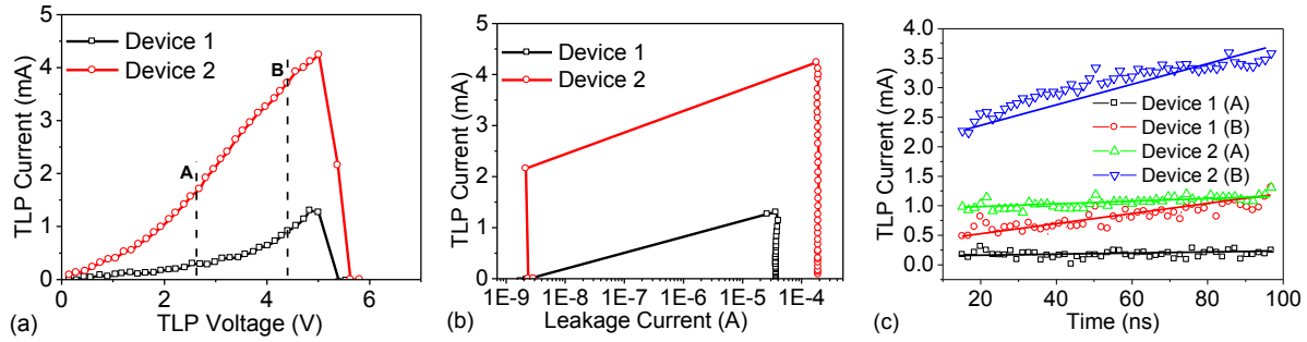
Figure 2: (a) TLP characteristics of suspended tubes (b) change in low-bias leakage with TLP current (c) Transient waveforms at two different TLP voltages marked in (a). Note that current remains constant with time at bias point marked A , while at point B , it increases linearly with time.
