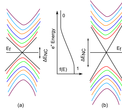
Figure 11: Sub-bands of (a) outer and (b) inner shells of a MWCNT. Note that the number of sub-bands smeared by Fermi-Dirac distribution decreases with decrease in diameter of the shell.
