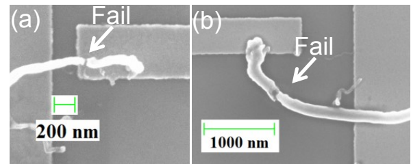
Figure 4: (a) SEM image of (a) Device 1 & (b) Device 2 after shell by shell failure. Both the devices are suspended between metal electrodes. Note that the devices have failed near contact, indicating ballistic transport through the tube.
