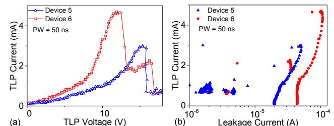
Figure 9: TLP characteristics of substrate-supported MWCNTs, excited by pulses of width 50 ns. Note that leakage current increases before showing shell-by-shell breakdown.
