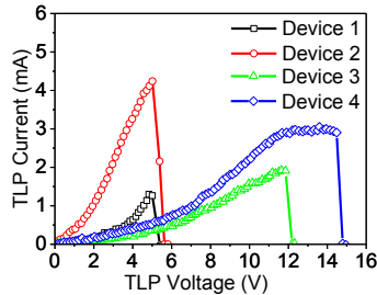
Figure 8: Comparison of TLP characteristics of suspended tubes (Device 1 and Device 2) with substrate supported tubes (Device 3 and Device 4). Compared to suspended tubes, the substrate supported tubes show higher breakdown voltage and carry relatively less amount of current.
