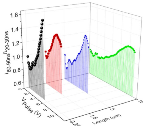
Figure 12: Change in relative increase in ESD current with pulse voltage and tube's length.
