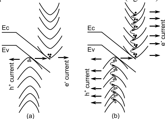
Figure 5: Occupancy of sub-bands at (a) t = 0^+ and (b) t \geq t_{\text{equilibrium}} . Band diagrams are shown for interface at the cold contact.
