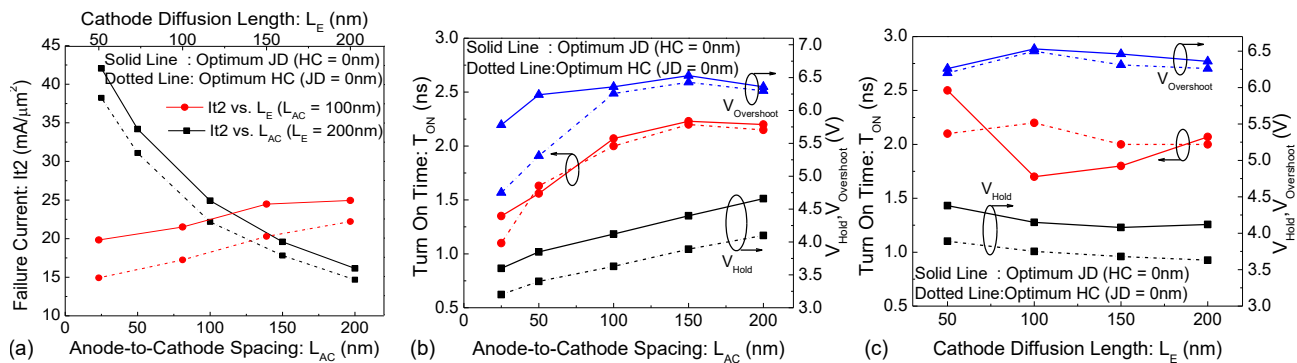
Figure 14: Design scalability of proposed DFSCR. Failure current ( It_2 ), holding voltage ( V_{Hold} ), turn-on time ( T_{ON} ) and voltage overshoot ( V_{Overshoot} ) as a function of Anode-to-Cathode spacing ( L_{AC} ) and Anode/Cathode diffusion length ( L_E ). The trends were extracted using 3D TCAD simulation setup, at injected stress current equivalent to 90% of the respective It_2 .
