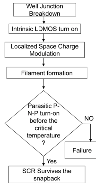
Fig. 6: Flow chart summarizing the Series of physical events that occur in LDMOS-SCR, that are critical for understanding the Power Scalability problem.
