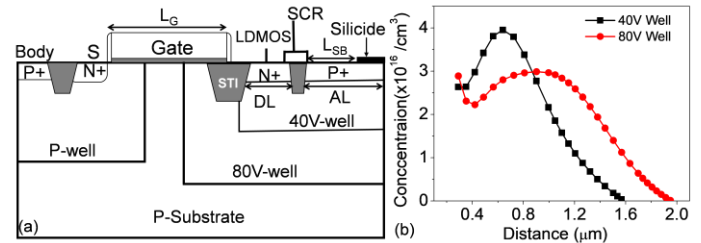
Fig. 1: (a) Cross-sectional view of LDMOS-SCR. To extract intrinsic LDMOS characteristics of LDMOS-SCR design, P+ (in N-Well) terminal was left floating. (b) Doping profiles of two different wells used in this work for obtaining 40 and 80 Voltage classes.
