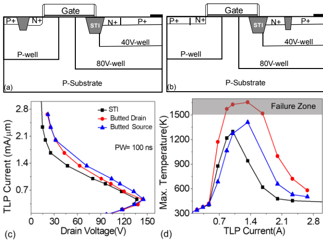
Fig. 10: device Cross-sections for Butted (a) Drain (b) Source. (c) Simulated (3D) TLP I-V characteristics LDMOS-SCR with STI isolation, butted configurations at source and drain. (d) Lattice temperature plotted a function injected current. Butted configuration at drain degrades P-N-P turn on, and at source slows down N-P-N, causes severe power scalability problems. The lattice temperature reaches to critical temp. Even with 100 ns Stress.
