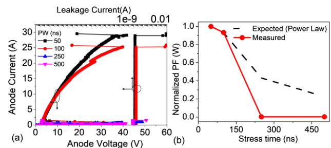
Fig. 2: (a) Measured TLP I-V characteristics LDMOS-SCR device for different stress pulse widths along with leakage data. (b) Normalized power to failure as a function TLP Stress time. Device stressed beyond 100ns duration are observed to fail during the snapback. Note that these TLP measurements are performed with the high impedance Setup that causes the SCR to experience the current values near snapback.
