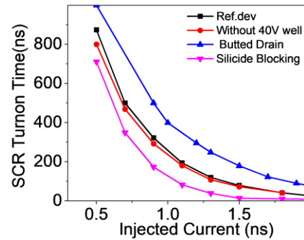
Fig. 13: SCR Turn-on time a function of injected current, for different designs under Investigation. Drain side butted configuration shows slowest SCR turn on and worst power scalability behavior. Whereas Silicide Blocked on AL shows fastest SCR turn on and best power scalability trends.
