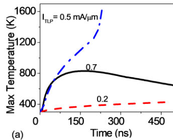
Fig. 4: Simulated transient temperature plotted as a function of stress time for different injected current near the snapback. Lower current values temperature increases linearly with time. For moderate current values near snapback, the lattice temperature abruptly increase and reaches the critical temperature for device failure, however device is found to survive the higher current levels with reduction in temperature beyond a peak value.
