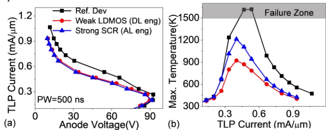
Fig. 7: simulated (a) TLP I-V (b) Maximum temperature plotted as a function of current for 40V LDMOS-SCR devices with AL and DL engineering. Increasing AL (emitter of P-N-P) improves SCR action and reducing DL Weakens the LDMOS action. Peak temperature can be safely limited below Critical value and hence power scalability is achieved.
