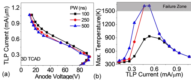
Fig. 3: Simulated 3D TCAD simulated (a) TLP I-V (b) Maximum temperature plotted as a function of current for different pulse widths. Temperature near snapback increases beyond critical temp for PW>100ns.
