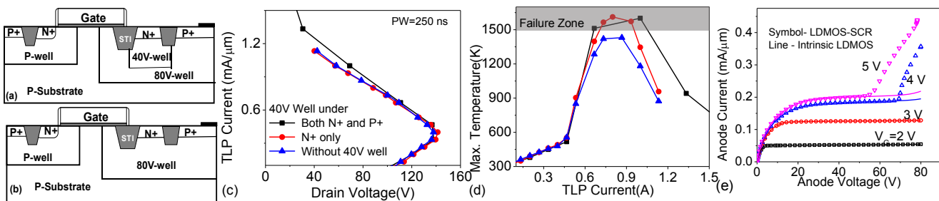
Fig. 11: Device cross-section of 40V Well profile changes (a) Underneath only N+ (b) W/o 40V well (c) LDMOS-SCR TLP I-V characteristics and (d) Maximum Lattice temperature vs injection current for different 40V well placements inside 80V well. 40V well increases the doping near the surface in the 80V well. If it is under both N+ & P+, yields worst case condition with larger failure window. 40V well under only N+ though reduces the failure window; cannot improve the power scalability. If 40V well is not implanted the failure window disappears for 250 ns PW, improved Power scalability but causes strong SCR action in the on-state (e)
