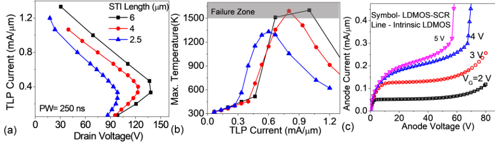
Fig. 9: TLP I-V characteristics LDMOS-SCR for different STI lengths (b) Lattice temperature plotted a function injected current. Reduction in STI length reduces I_{t1} , V_{t1} and causes early filament formation. However, the smaller operating voltage attributed to reduced anode cathode distance, ensures that self-heating in filament do not reach critical temperature. However, reducing STI length for increasing power scalability has negative implications on on-state performance (Reduction in on-state breakdown voltage).
