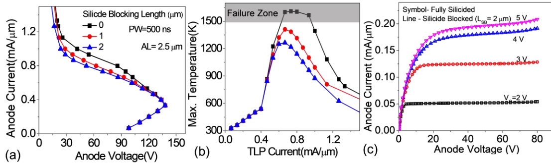
Fig. 12: (a) TLP I-V Characteristics of LDMOS-SCR (b) Maximum Lattice temperature plotted as function Silicide blocking length. Increasing Silicide Blocking on P+ found to reduce the lattice temperature, during snapback. Improvement in power scalability with silicide blocking is purely a 3D phenomenon, the peak lattice temperature from 2D Simulations do not change (data not shown). (C) DC I-V characteristics showing no influence on on-state characteristics.
