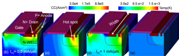
Fig. 5: Conduction current density (b & d), Lattice temperature (c & e) for ITLP of 0.5 and 1 respectively. The temperature shoots up attributed the LDMOS filament for current of 0.5 (b & c). However, for larger current SCR turn-on (d & e) and filament spreading causes safe conduction.
