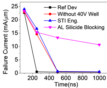
Fig. 14: Final Power Scalability trends for different designs Investigated.
