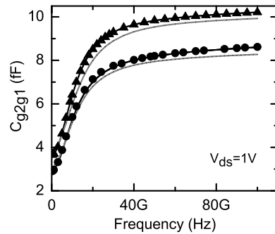
Fig. 6 Frequency response of C_{g2g1} at V_{gs1} = 1 V. Circle represents V_{gs2} = 0.7 V and triangle represents V_{gs2} = 0.9 V. Black line represents exact solution of (10), while the gray line represents 4-point collocation method based solution
