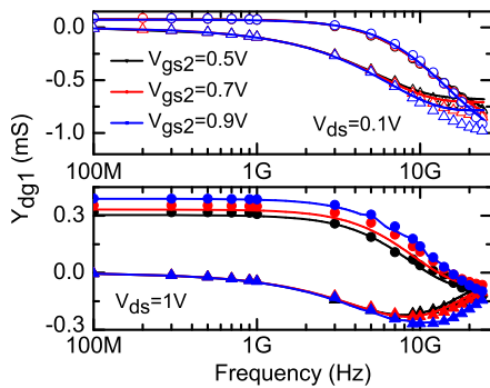
Fig. 5 Relationship between Y_{dg1} in both linear and saturation region. Line represents the model and symbol represents TCAD data. In all the plots V_{gs1} is kept at 1 V. Saturation f_i values are 2.36 GHz, 2.6 GHz, 2.85 GHz for V_{gs2} = 0.5 V, 0.7 V, 0.9 V respectively, while the linear f_i remains almost at 0.478 GHz for all V_{gs2}
