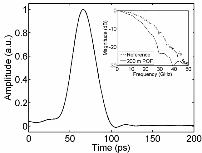
Figure 27. Deconvolved response of 200 m POF showing a 29 ps FWHM. Inset: Corresponding frequency response.
